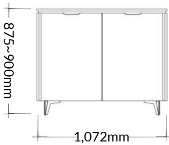
2 Door (487mm)
