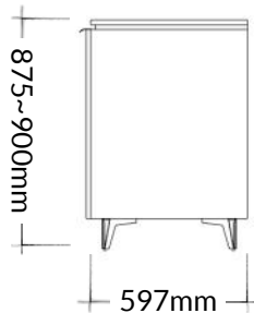
Side Elevation
